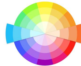
complementary colours
