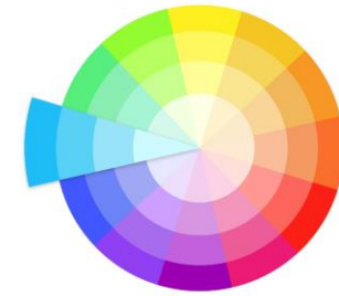
monochrome colours
